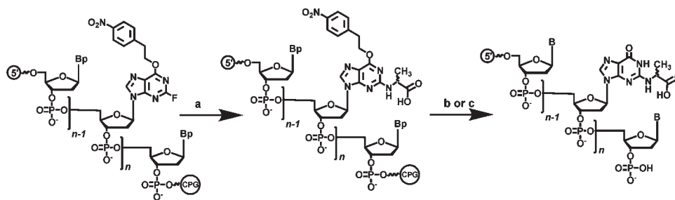
FIGURE 1: Synthesis of oligonucleotides containing (R)- or (S)-CEdG. Conditions: (a) D- or L-alanine, K_2CO_3 , H_2O/N -methylpyrrolidone, 50 °C, 48 h; (b) concentrated NH_4OH , 55 °C, 4–7 days; (c) DBU/ C_5H_5N , room temperature, 18 h. Bp indicates protected DNA bases.
