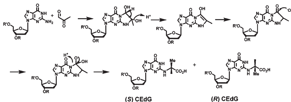
Scheme 1: Proposed Mechanism of Formation of ( R,S )-CEdG via the Addition of Methylglyoxal to N 1 and N 2 of 2'-dG a
