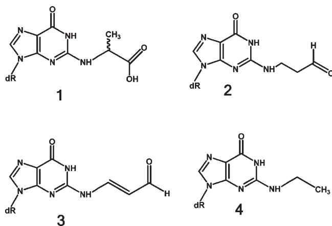
FIGURE 6: N2-substituted acyclic aldehyde adducts of 2'-deoxyguanosine: 1, ( R,S )-CEdG; 2, N^2 - \gamma -(oxo)-PdG; 3, N^2 -3-oxoprenyl-M1dG; 4, N^2 -ethyl-dG. Adducts 2 and 3 are in equilibrium with the corresponding N1, N2 cyclic forms \gamma -OH PdG and M1dG, respectively.
