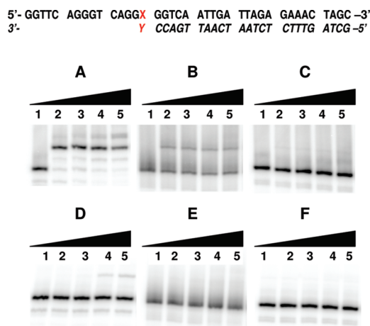
FIGURE 5: Primer extension from 3'-CEdG catalyzed by Kf^- . For lanes 1–5, [dCTP] in \mu M: 0, 2.5, 25, 250, and 2500. (A) X = C, Y = G; (B) X = C, Y = (R)-CEdG; (C) X = C, Y = (S)-CEdG; (D) X = A, Y = G; (E) X = A, Y = (R)-CEdG; (F) X = A, Y = (S)-CEdG.
