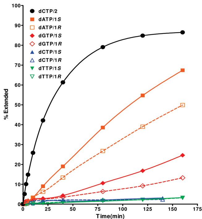
FIGURE 3: Progress curves for the incorporation of dNTPs opposite (R)- and (S)-CEdG in template DNA catalyzed by Taq polymerase. A control reaction showing the time course for dCTP incorporation opposite dG within the same sequence environment is provided for comparison (black dots).
